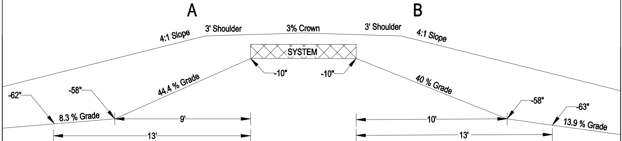
Cross Section for field data shown on Figure 3a.
